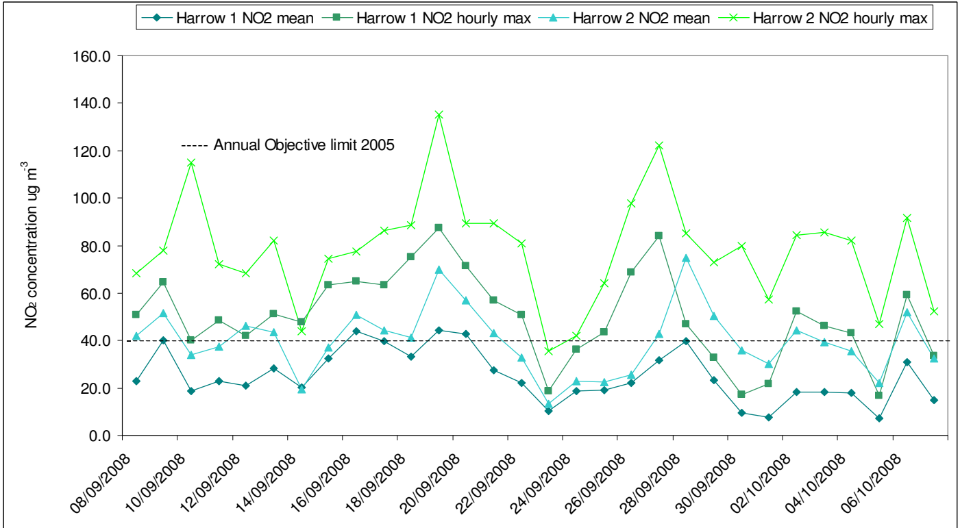
Nitrogen Dioxide (NO 2 ) concentrations (µg m -3 ) from Harrow 1 (Background) and Harrow 2 (Roadside) continuous monitoring stations from 8-Sep-2008 to 7-Oct-2008.
