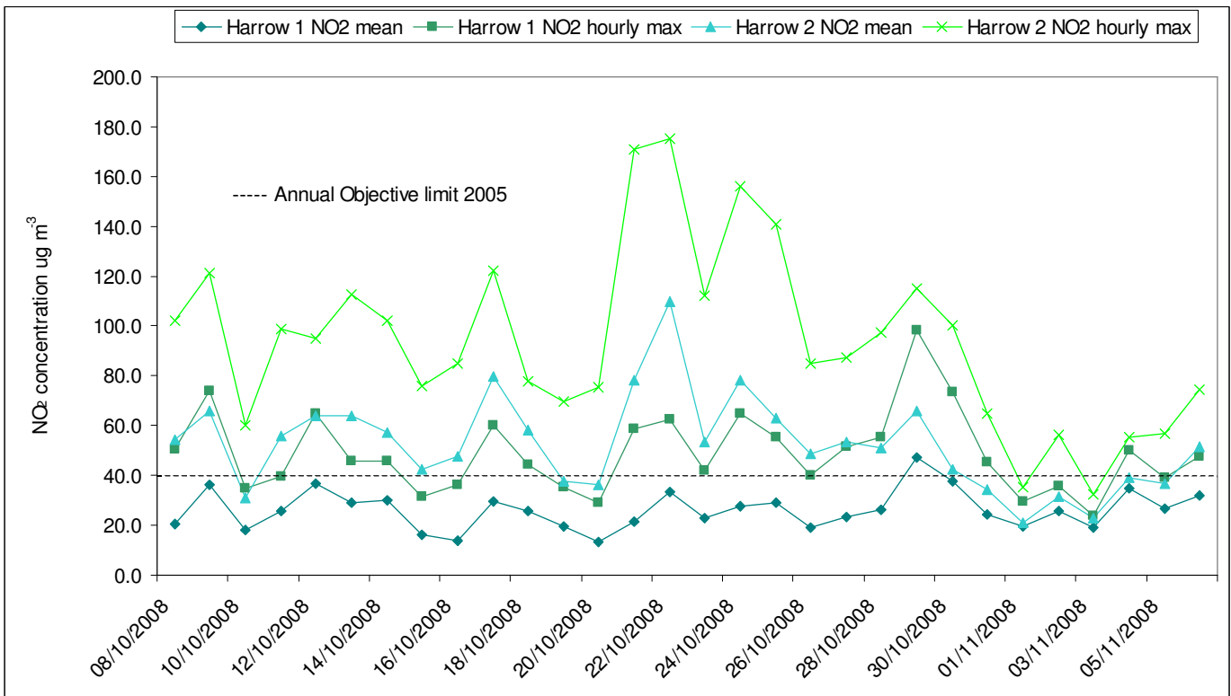
Nitrogen Dioxide (NO 2 ) concentrations (µg m -3 ) from Harrow 1 (Background) and Harrow 2 (Roadside) continuous monitoring stations from 8-Oct-2008 to 6-Nov-2008.
