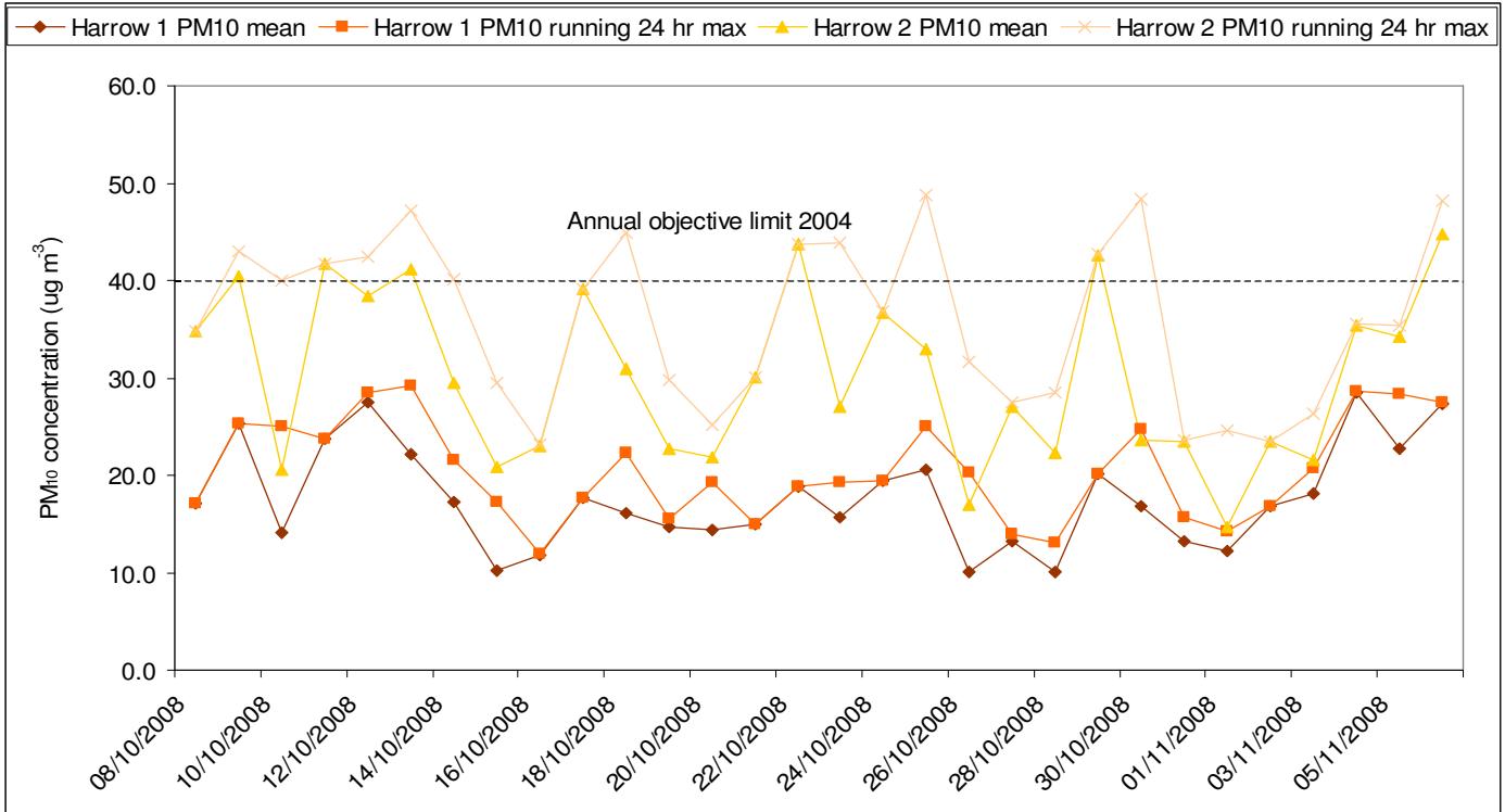
Particulate (PM 10 ) concentrations (µg m -3 ) from Harrow 1 (Background) and Harrow 2 (Roadside) continuous monitoring stations from 8-Oct-2008 to 6-Nov-2008.
