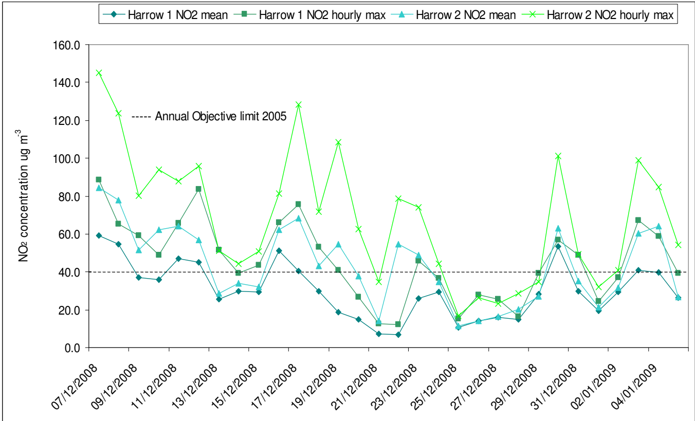
The NO 2 mean concentrations are daily mean figure and the NO 2 hourly max are the maximum figure in an hour for the 24 hour period.
