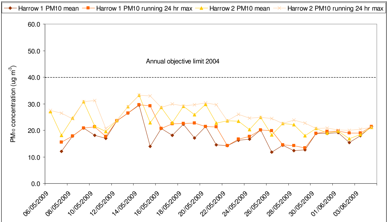
Particulate (PM 10 ) concentrations (µg m -3 ) from Harrow 1 (Background) and Harrow 2 (Roadside) continuous monitoring stations from 6-May-2009 to 4-Jun-2009.
