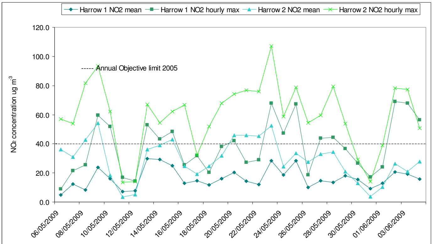
The NO 2 mean concentrations are daily mean figure and the NO 2 hourly max are the maximum figure in an hour for the 24 hour period.
