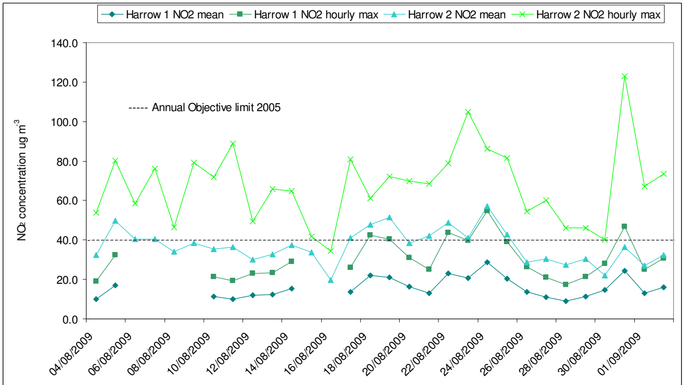
Nitrogen Dioxide (NO 2 ) concentrations (µg m -3 ) from Harrow 1 (Background) and Harrow 2 (Roadside) continuous monitoring stations from 4-August-2009 to 2-September-2009.
